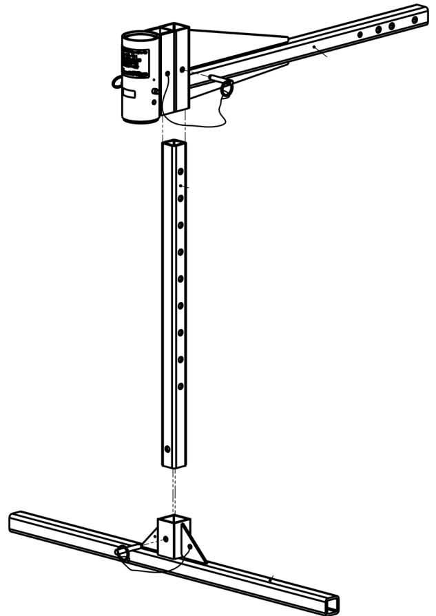
EXPLODED VIEW
